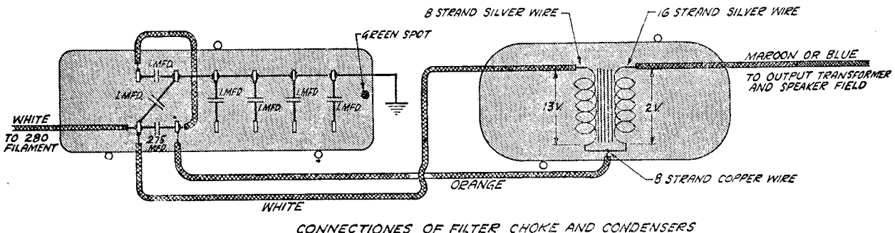
CONNECTIONS OF FILTER CHOKE AND CONDENSERS
